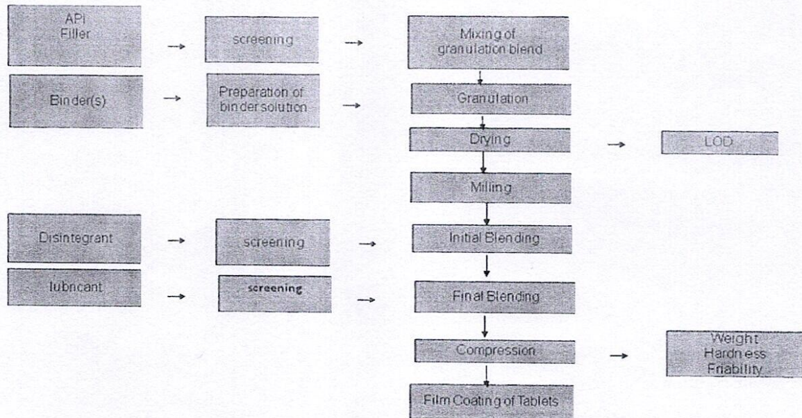
Fig.1: Unit operations for Tablet
